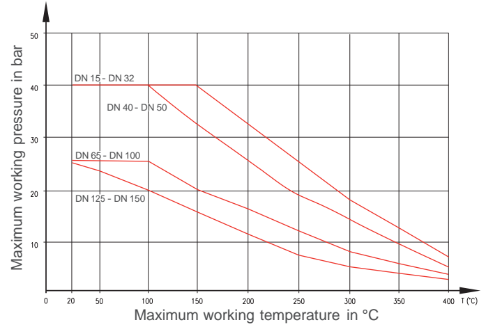
Metal Seat
