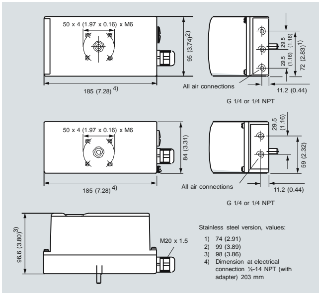
Makrolon and stainless steel enclosure (top), aluminum enclosure (center), Makrolon and aluminum enclosure (bottom), dimensions in mm (inch)
