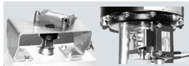
NCS for part-turn actuator (6DR4004-NN10) mounted with mounting console (left) and NCS for linear actuator ≤ 14 mm (0.55 inch) (6DR4004-NN20) mounted with actuator-specific mounting solution (right)
